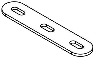
Mounting Plate 86x18x2mm 2x
